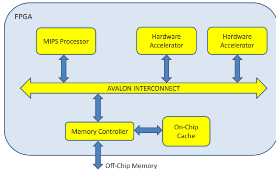
Figure 2: Target system architecture.
