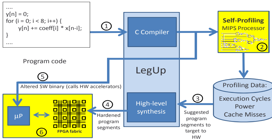
Figure 1: Design flow with LegUp.
