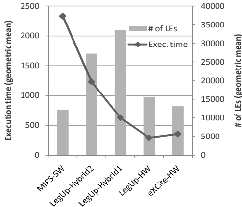
Figure 8: Performance and area results.
